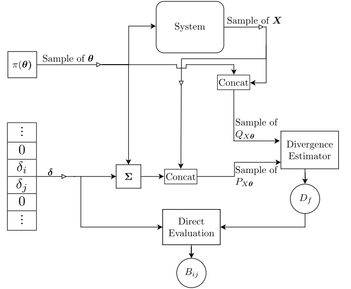
Figure 2. Procedure of the accelerated FINE for B-FIM estimation.
