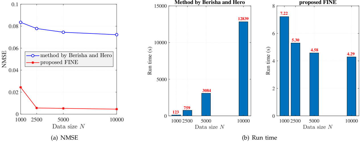
Figure 3. Estimation accuracy and computational complexity comparison for the case of deterministic \theta .
