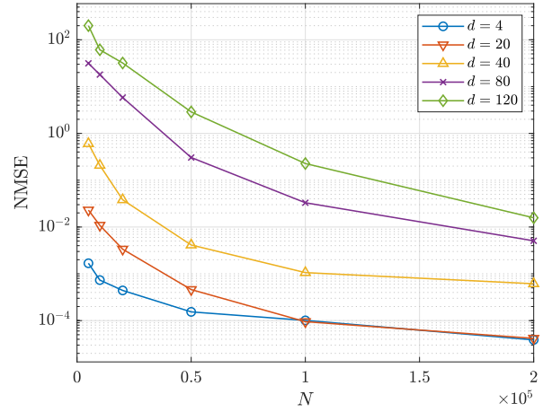
Figure 6. Accelerated FINE for high parameter dimensions.
