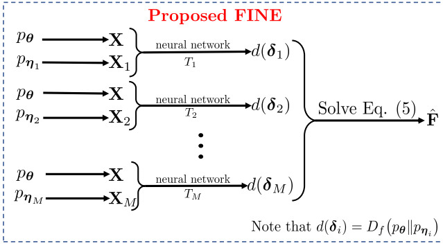
Figure 1. Illustration of the proposed FINE method.
