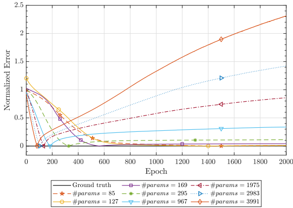
Figure 8. Estimation error versus \#params and training epoch for the test scenario in Section 5.1 with L = 1 , W = 40 , and N = 20000 .
