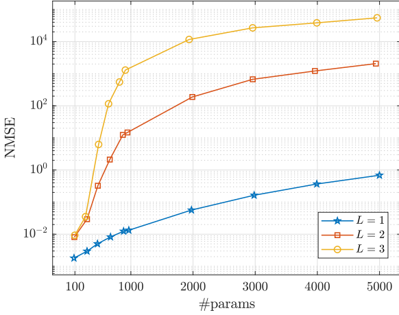
Figure 7. Effects of the neural network size with d = 40 and N = 10000 .
