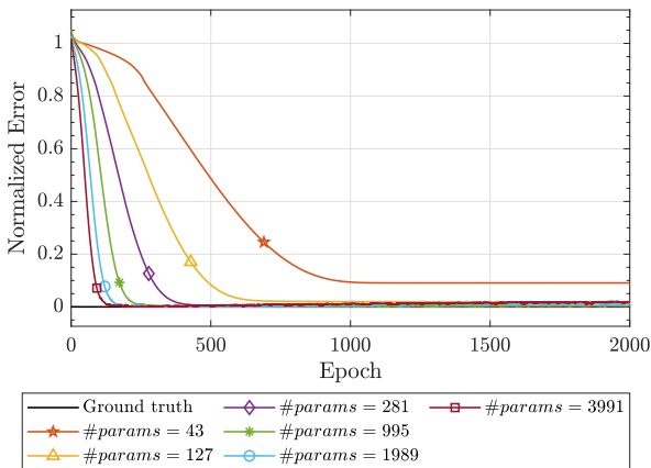
Figure 9. Estimation error versus \#params and training epoch for the test scenario in Section 5.2 with L = 1 , W = 12 , and N = 10000 .
