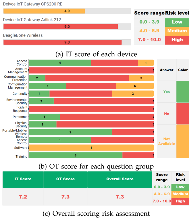
Figure 13: An example of risk assessment result using RA web-service for Vietnam.
