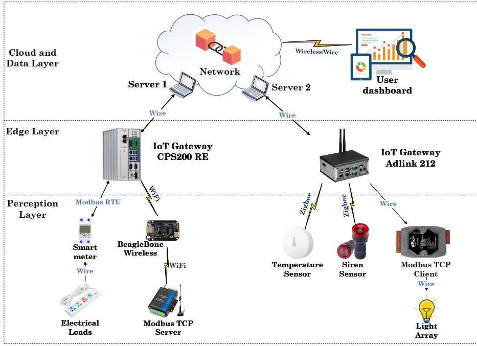
Figure 9: Our experimental model to simulate a real IIoT system.
