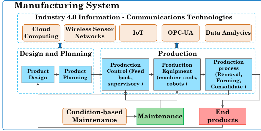
Figure 2: Manufacturing workflow in Industry 4.0 [16].
