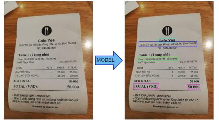
Fig. 1. The key information detection problem takes an image as an input and returns the location and type of key information in the image
