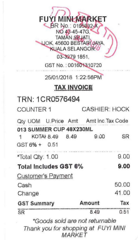
(a) SROIE [4]
