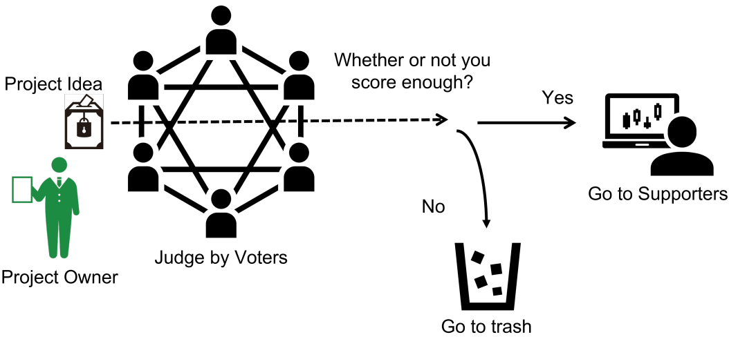
Figure 2. Proposal for a Decentralized Voting Method
