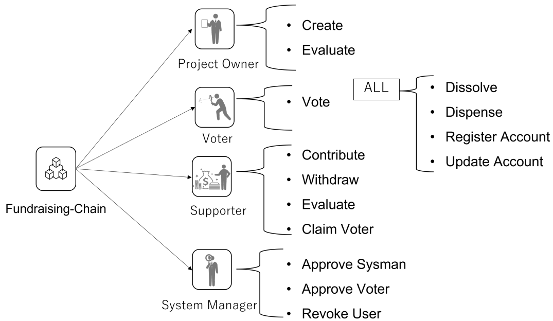
Figure 5. Main smart contracts of the proposed system
