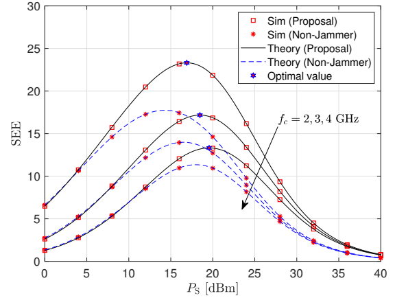
Figure 8. The SEE of the considered system versus the P_S for f_c = 2, 3, 4 and L = 30 .
