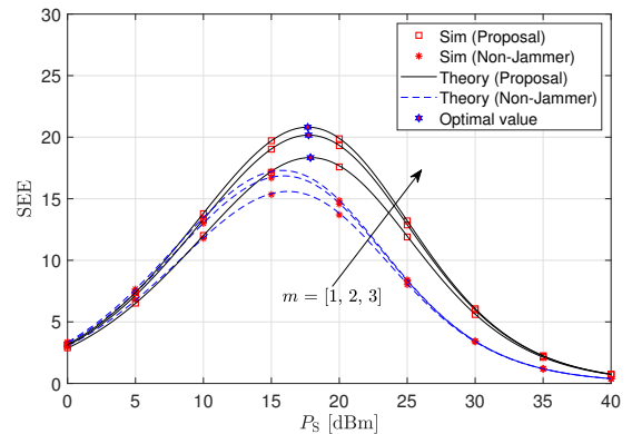
Figure 9. The SEE of the considered system versus the P_S for m = 1, 2, 3 and L = 20 .
