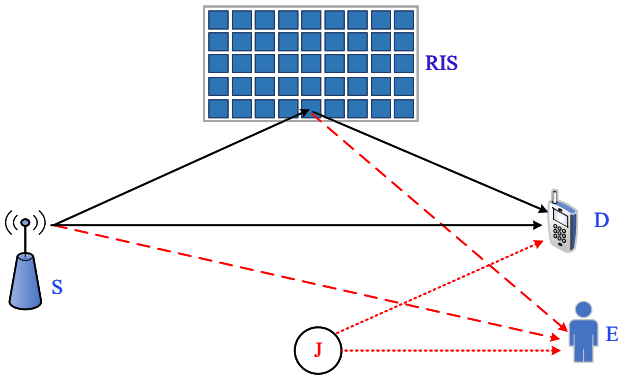
Figure 1. System model of the proposed RIS-Jammer-SISO communication system in the presence of an eavesdropper.
