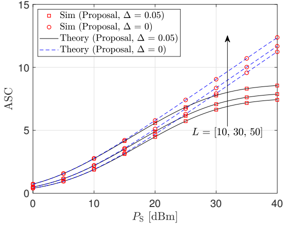
Figure 6. The impact of \Delta on ASC of the considered system with L = 10, 30, 50 and f_c = 3 GHz.
