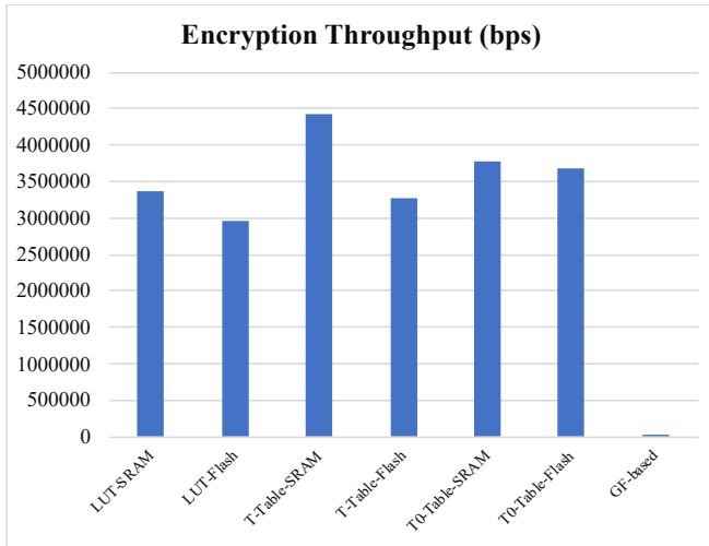
Fig. 1. Encryption throughput for each SM4 implementation
