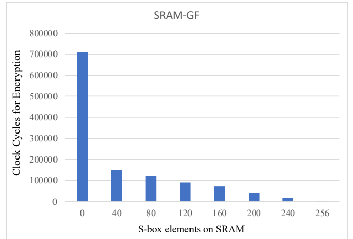
Fig. 3. Encryption latency for hybrid SRAM-GF S-box
