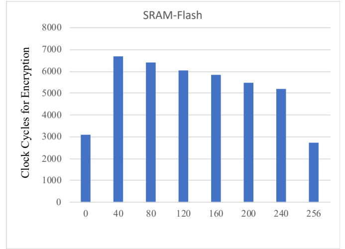
Fig. 2. Encryption latency for hybrid SRAM-Flash S-box
